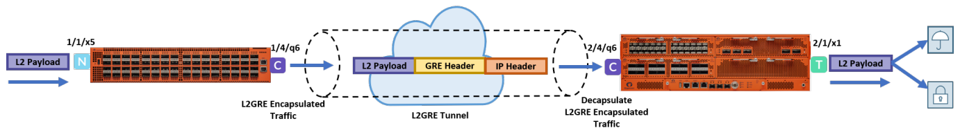
Figure 29 L2GRE Tunnel Encapsulation and decapsulation
