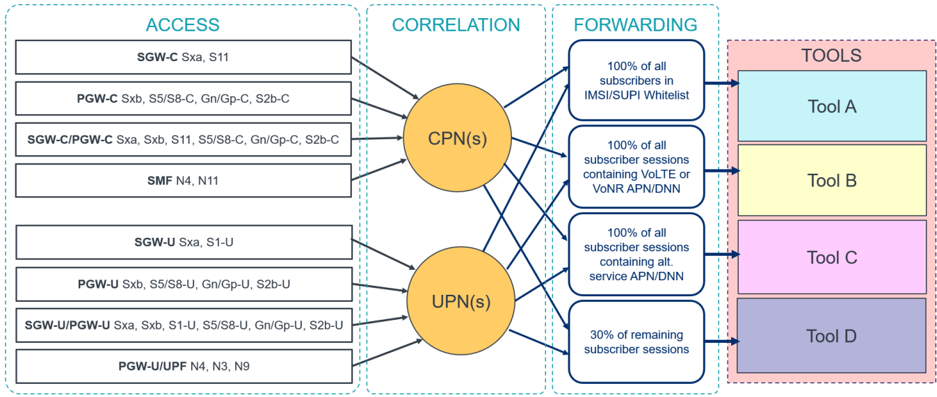
Figure 21 CUPS Traffic Visibility Solution
