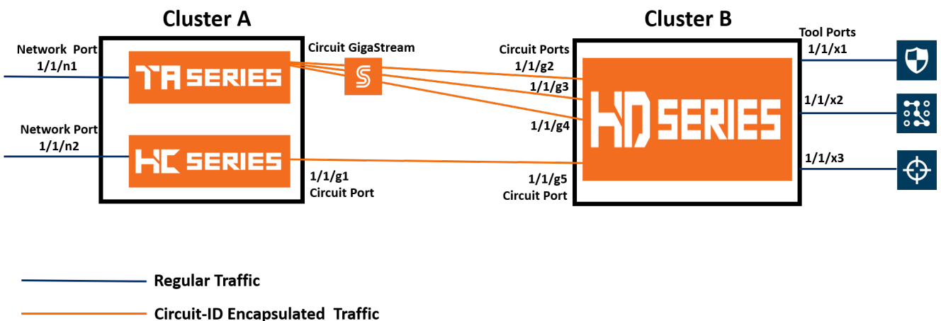
Figure 28 Circuit Flow Mapping®
