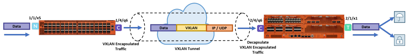
Figure 30 VXLAN Tunnel Encapsulation and Decapsulation
