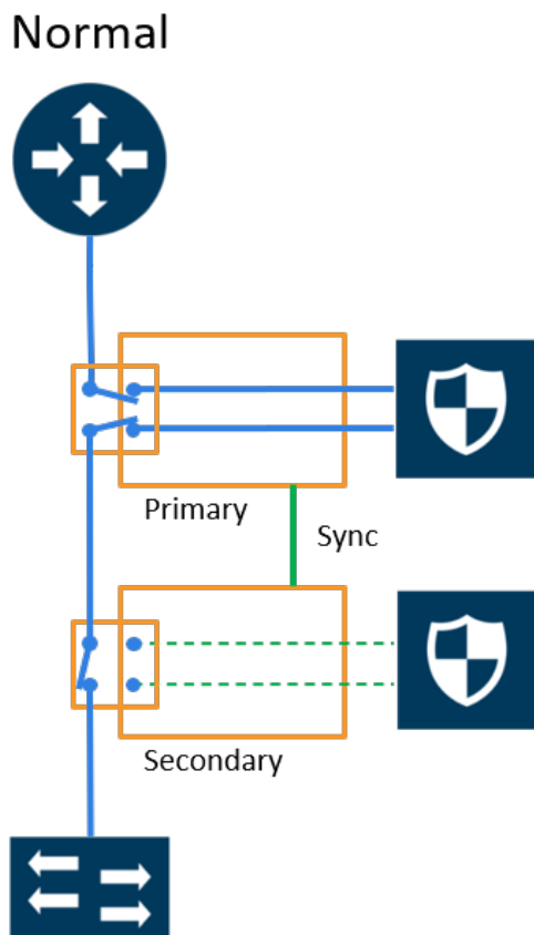
Figure 22 Traffic Flows Through Node with Primary Role
