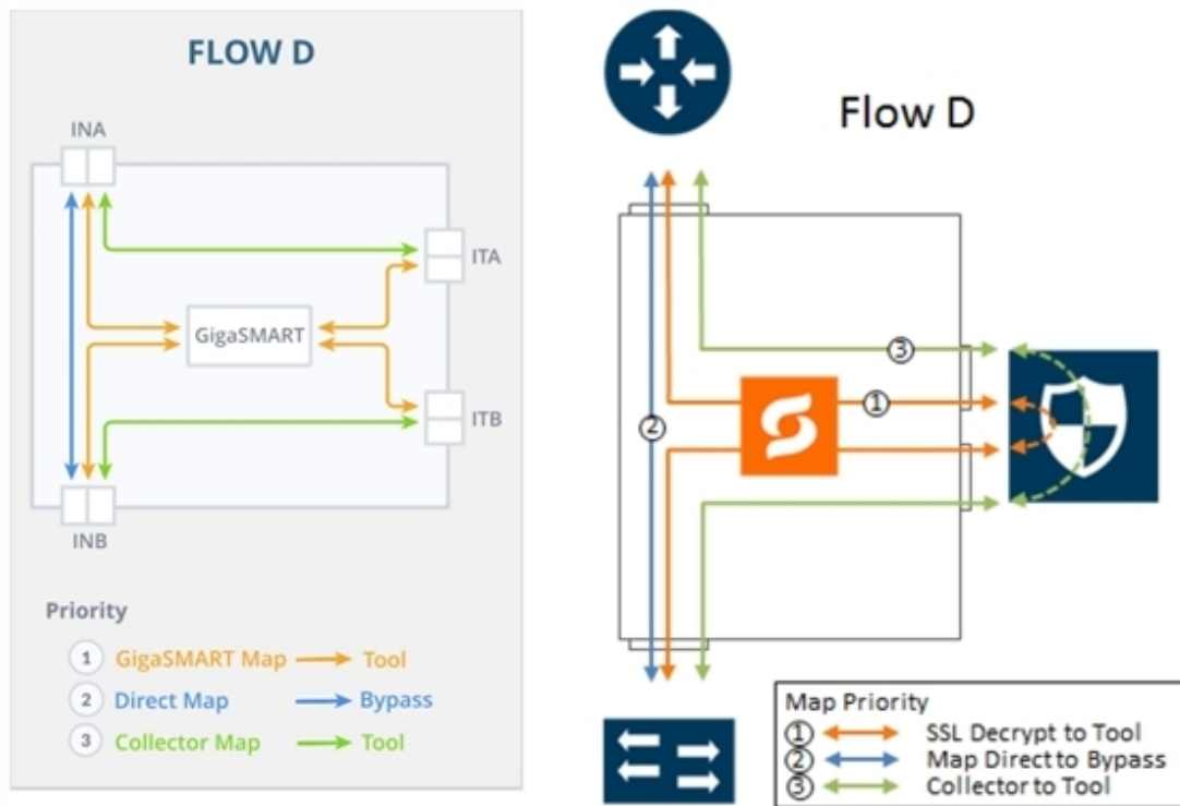
Figure 53 FLOW D Views
