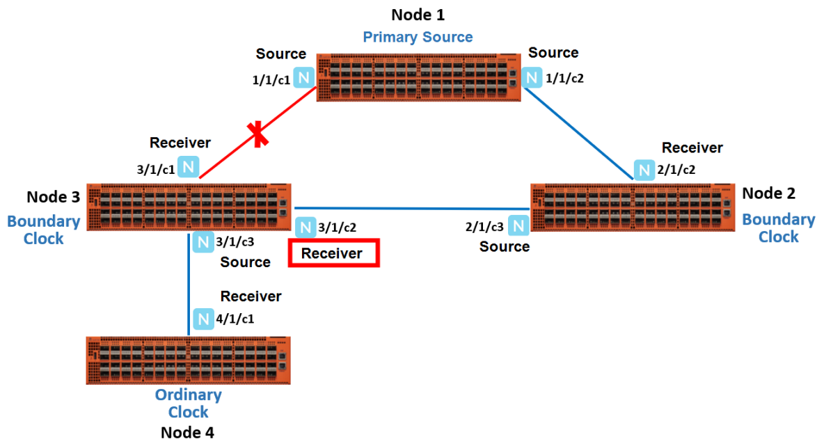
Figure 28 PTP State Transition
