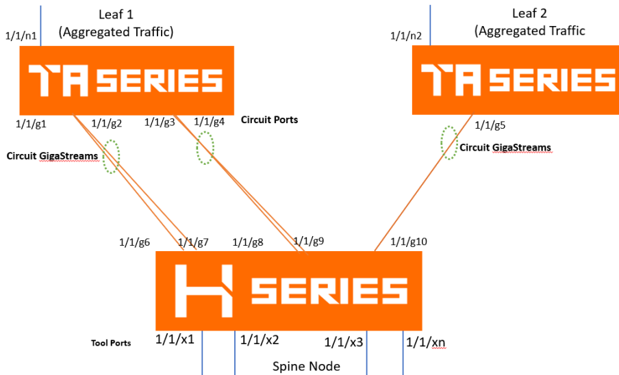
Figure 34 Circuit GigaStreams in Fabric Maps
