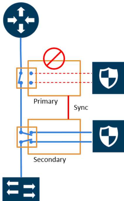
Figure 23 Traffic Flows Through Node with Secondary Role after Primary is Lost
