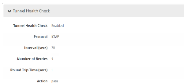
Figure 138 Configure ICMP Health Check Parameters
